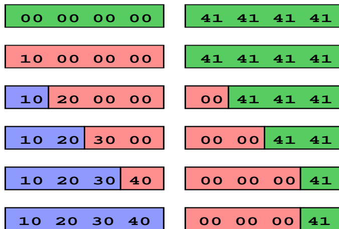
Figure 1: Four stage overwrite of an address
